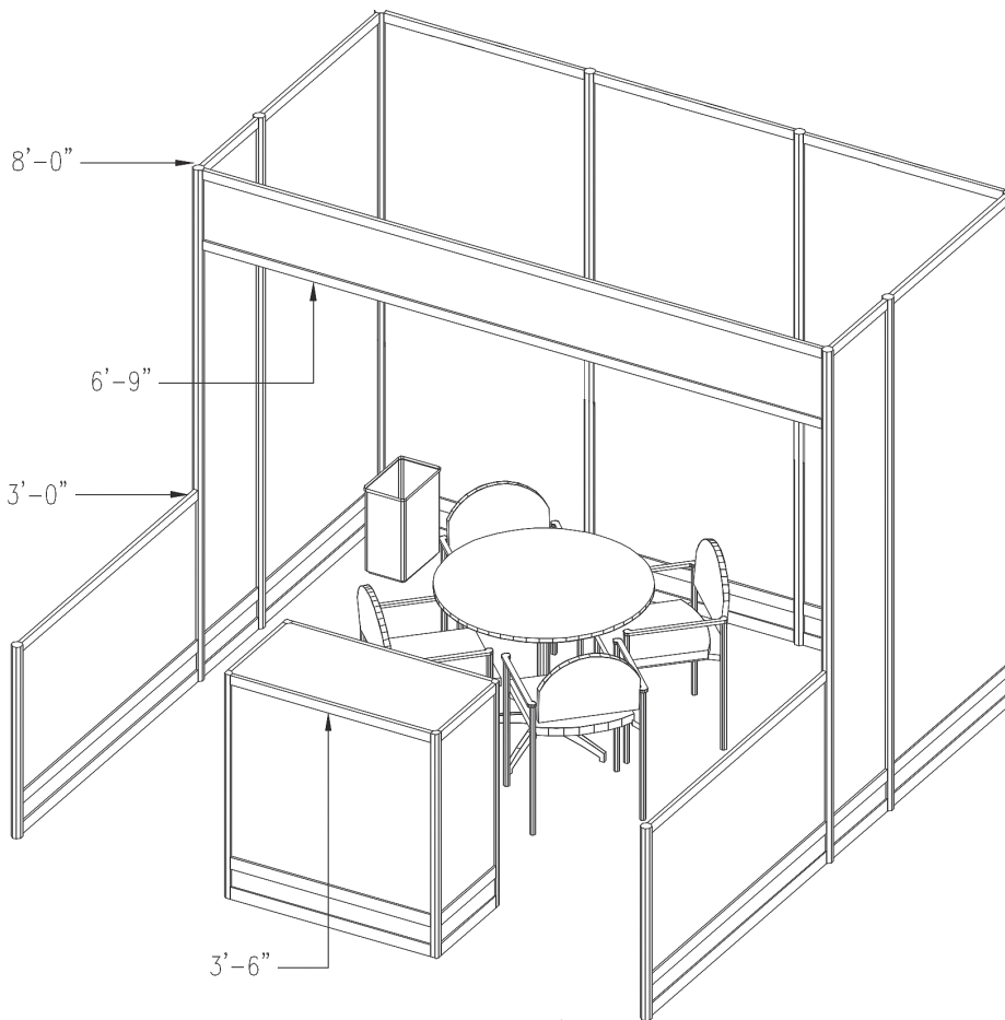
PERSPECTIVE VIEW Not To Scale
